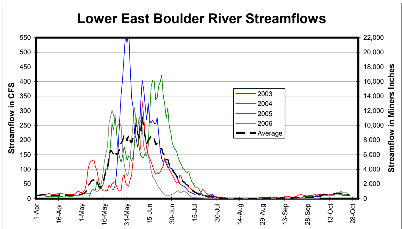
Figure B-4. Streamflows for the lower East Boulder River gage (2003-2006).
