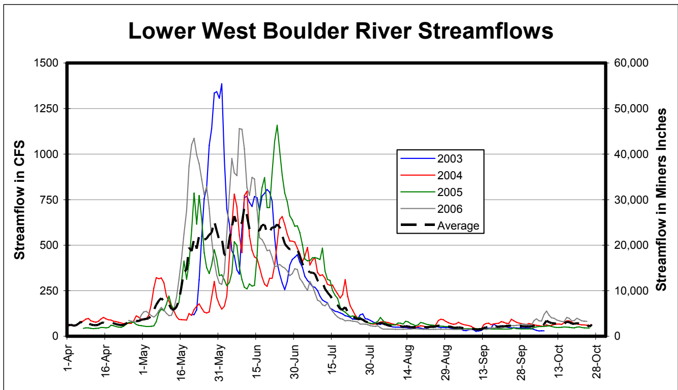
Figure B-6. Streamflows for the lower West Boulder River gage (2003-2006).
