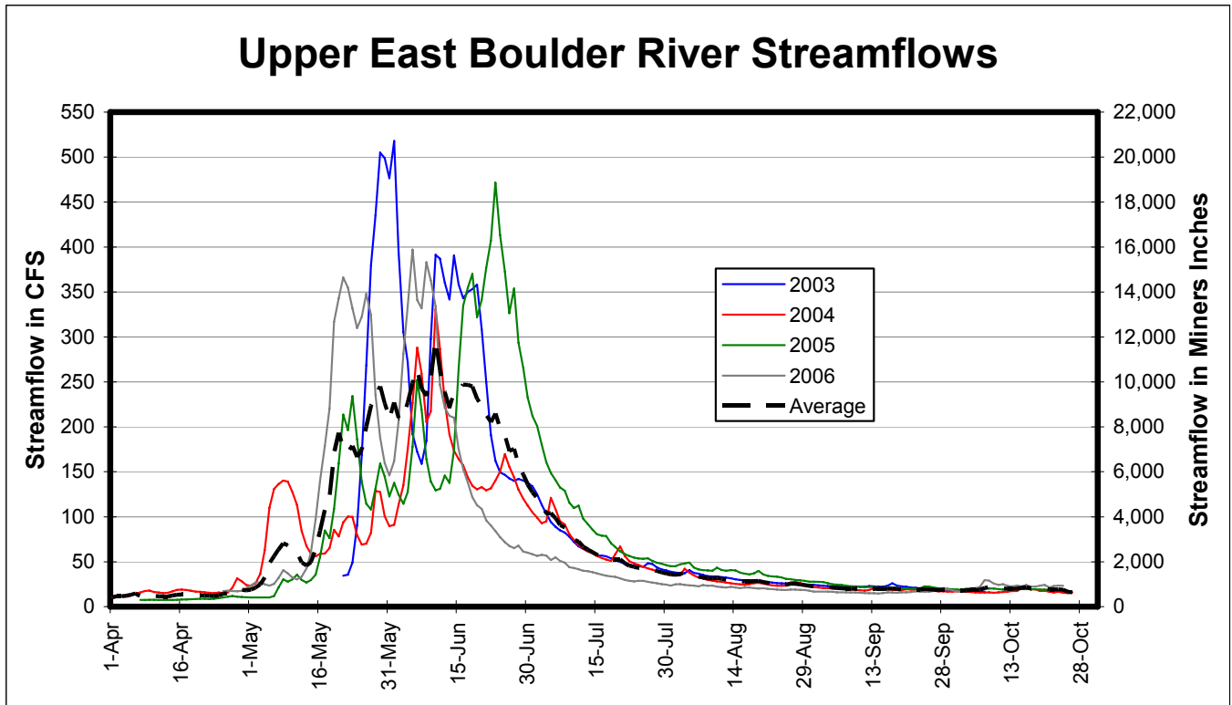
Figure B-3. Streamflows for the upper East Boulder River gage (2003-2006).
