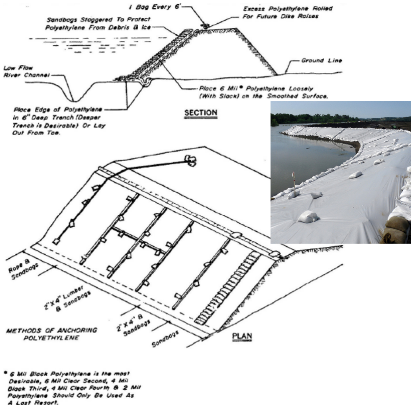
Figure 16: Placement of Polyethylene Sheeting Slope Protection in the Dry
