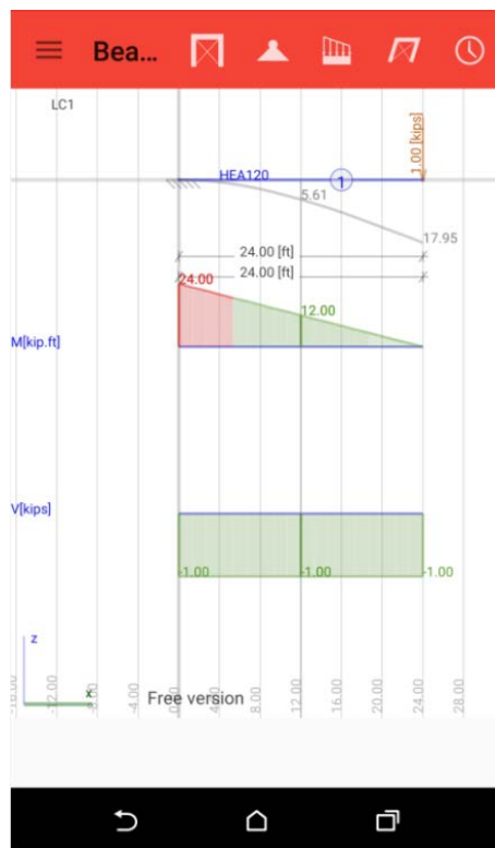
Figure 5 – LetsConstruct Beam Analysis
