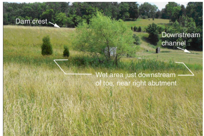
Figure 8. Presence of Phreatophytic Vegetation (willow tree and cattails) in a Seepage Location 200 feet below the Downstream Toe [2]
