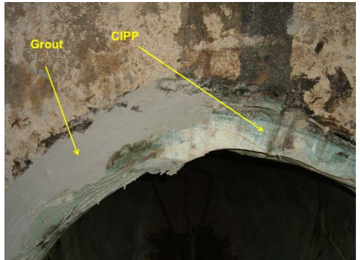
Figure 6 – Loose-fitting CIPP against Old CMP. (Portions of the pipeline had to be grouted.)
