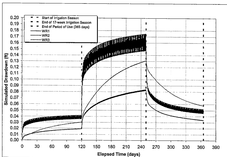
Simulated Drawdown in Nearby Wells (WR1 through WR3) Caused by Proposed Pumping in Salish Shores Wells 1 and 3 FIGURE 6b
