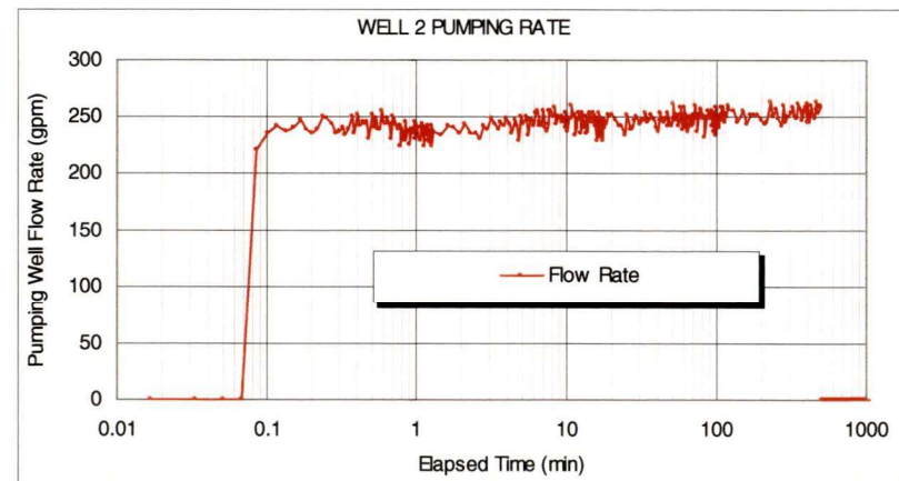
Pumping Well Flow Rates During Each Aquifer Test Salish Shores PWS Thompson Falls, Montana Appendix D
