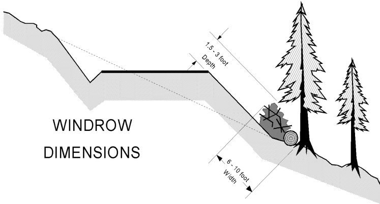
TYPICAL INSTALLATION
