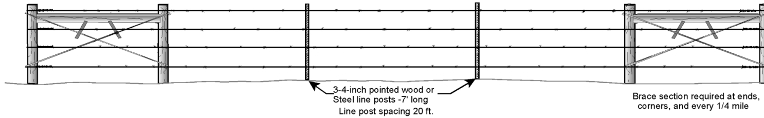
TYPICAL LINE FENCE SECTION
