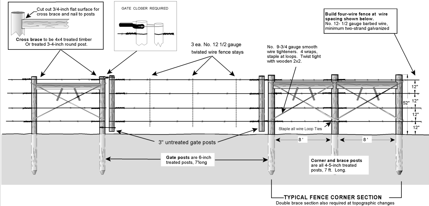
TYPICAL LINE FENCE SECTION
