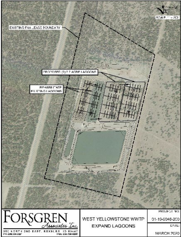
Figure 4-9: West Yellowstone WWTP Expand Lagoons
