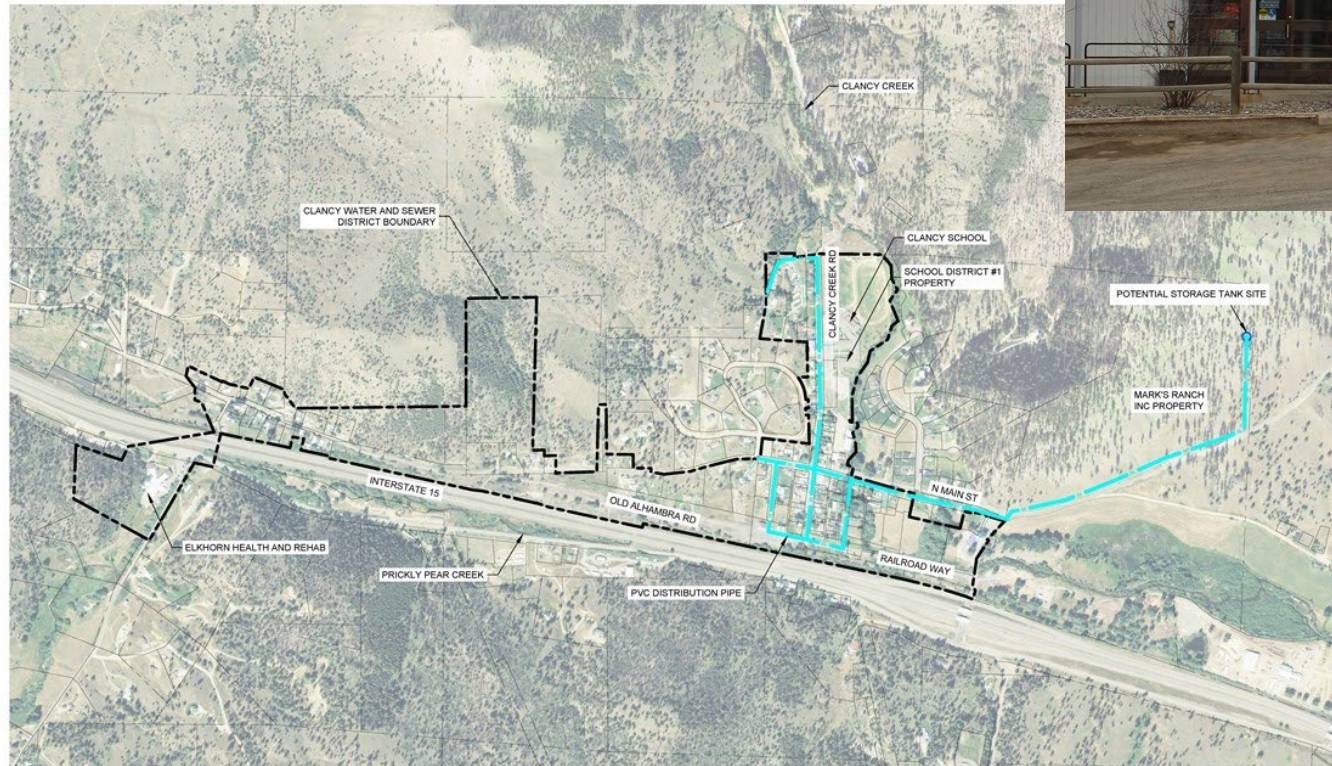
Figure 7-1 Clancy Phase 1 Water System Improvements
