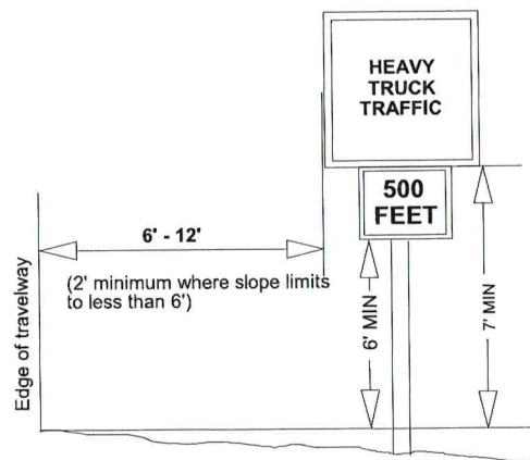
Figure 1: Sign Placement Dimensions
