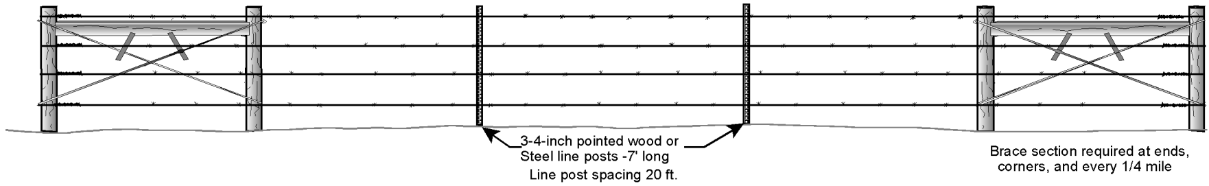
TYPICAL LINE FENCE SECTION
