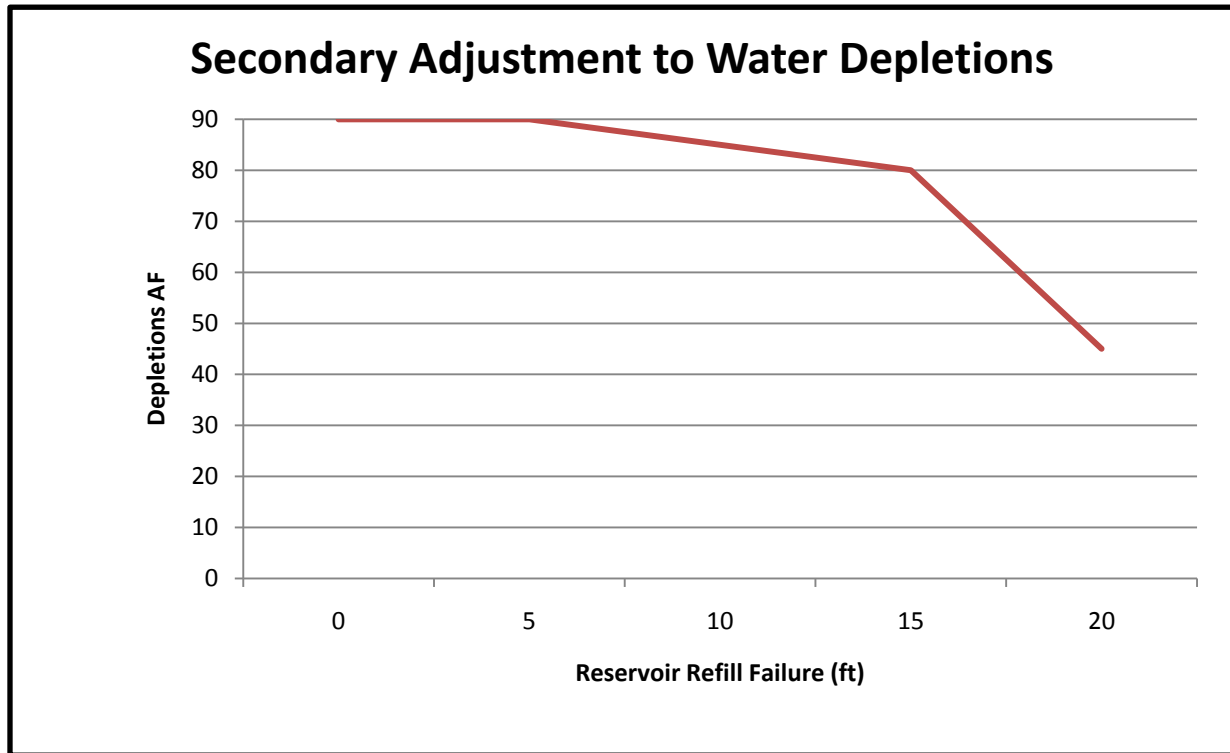
Figure 4. Secondary adjustment to the depletion volume based on the difference between the observed Hungry Horse Reservoir pool elevation and the Base Case elevation. This figure pertains to the period September through December
