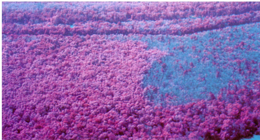
Figure 12.—The area in the red portion of this infrared photo was sprayed to kill forest tent caterpillar larvae. The unsprayed blue area was completely defoliated. The red area along the river in the lower right contains non-host tree species.
