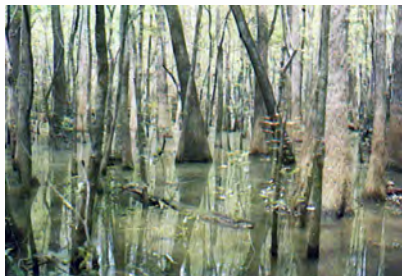
Figure 10.—Flooding of tupelo swamps during the larval feeding period prevents natural enemies from reaching the forest tent caterpillars.
