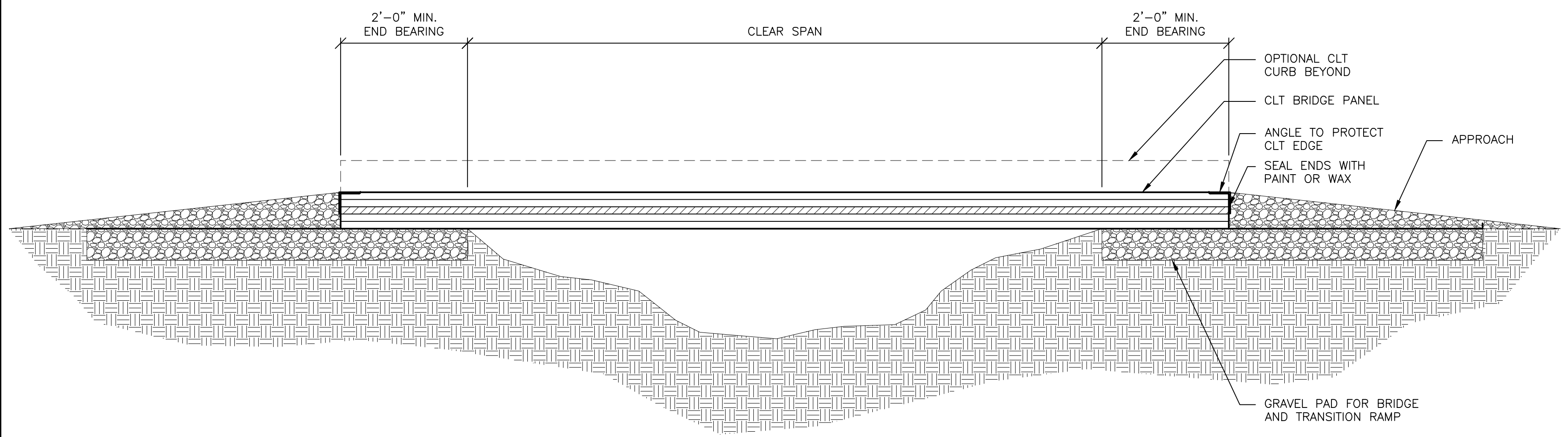
CLT BRIDGE PROFILE
