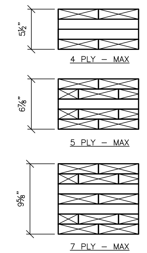
CLT LAYUP COMBINATIONS
