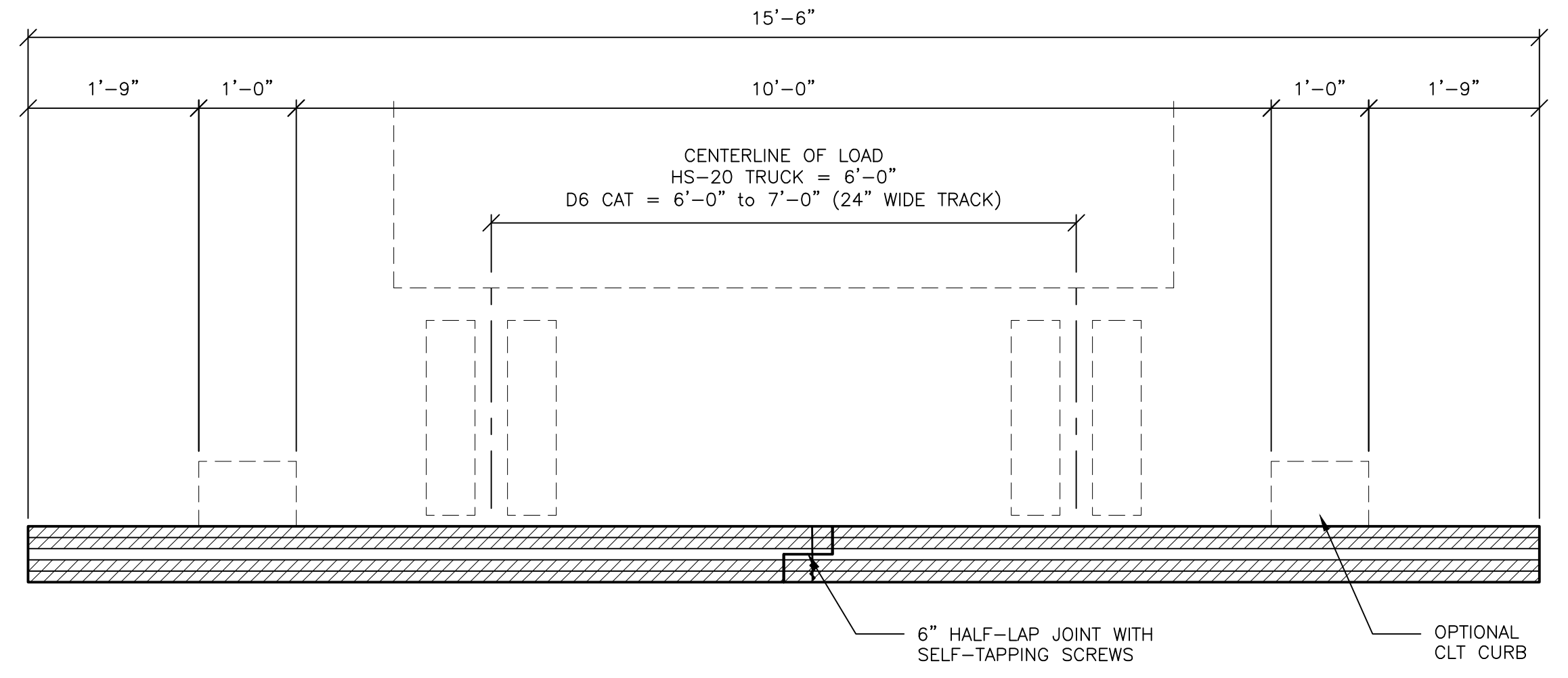
CLT BRIDGE SECTION
